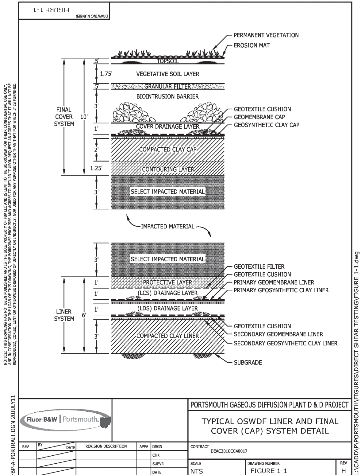
Figure 1-1. Typical OSWDF Liner and Final Cover (Cap) Systems Detail
